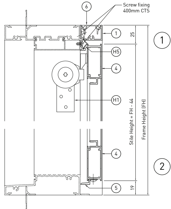
Open Outward Hinged Door Option
