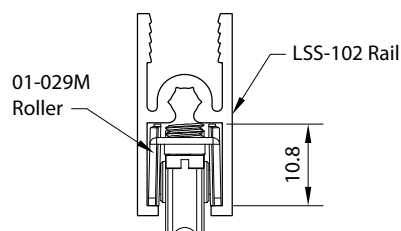
01-029M Roller in LSS-102 Rail
