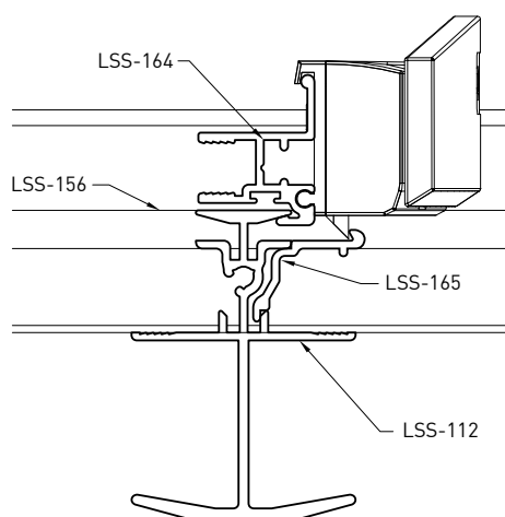
Lifestyle™ Sliding Window Sections with latch
